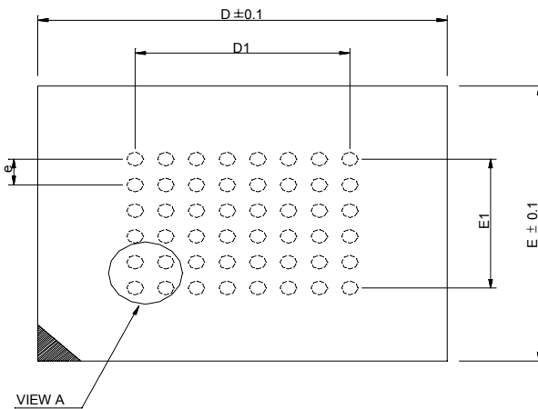
48 mini-BGA (8 x 10mm)
