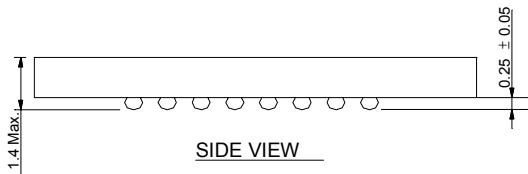
48 mini-BGA (6 x 8mm)
